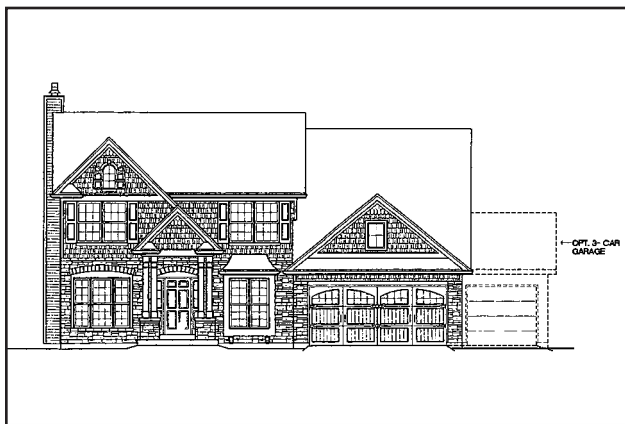
ELEVATION C
